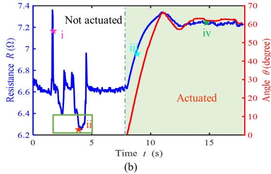
Fig. 10: (a) The snapshots of the autonomous bending finger that is triggered by external stimuli. i, ii, iii, iv are marked with stars in (b). (b) The resistance of the soft finger and the bending angle with respect to time.
